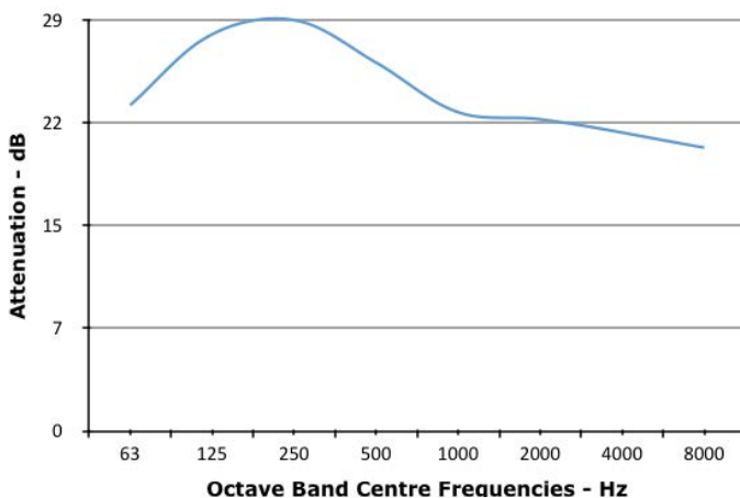
Typical Residential Spark Arrestor Silencer Attenuation
