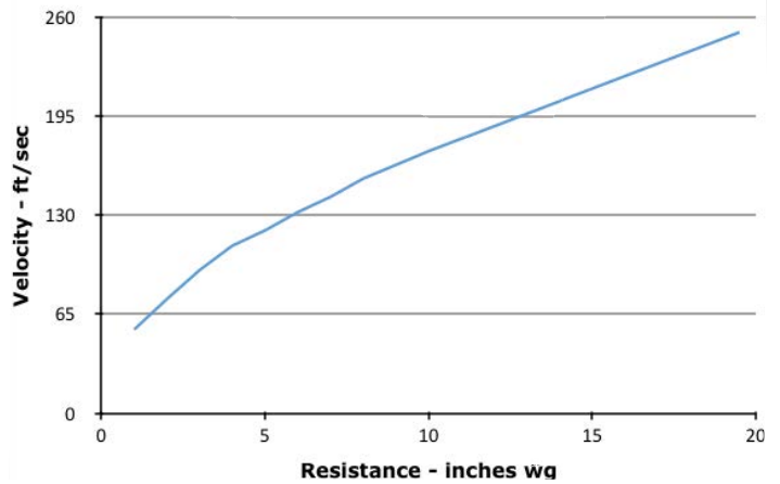
Typical Residential Spark Arrestor Silencer Velocity/Resistance
